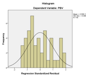
Gambar 2. Garfik Histogram
