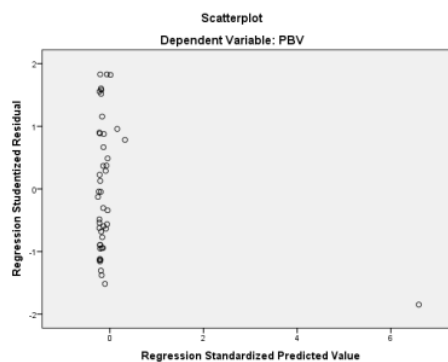
Gambar 2. Scatterplot
