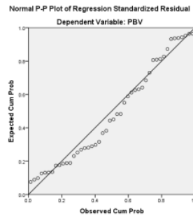
Gambar 3. PP-PLOT
